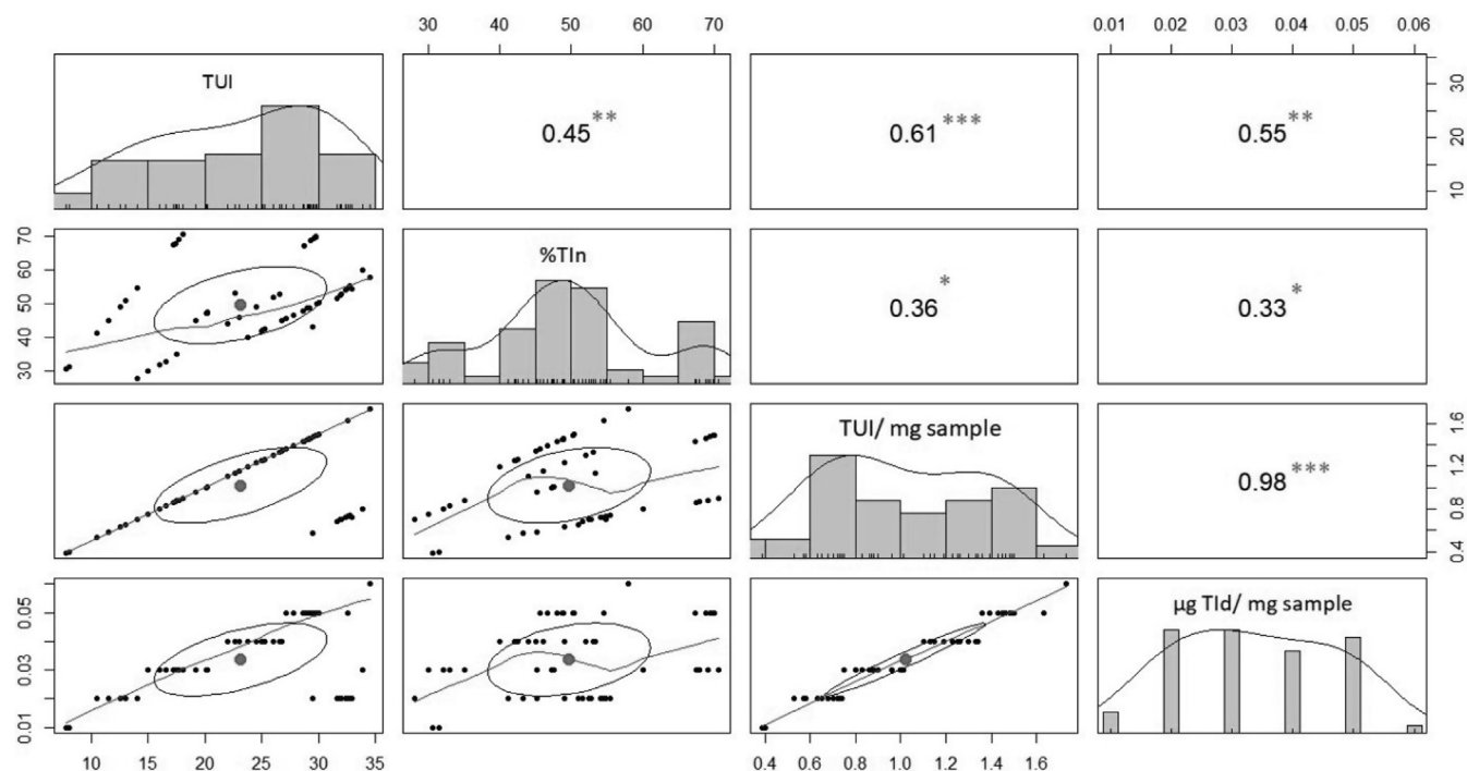
Fig. 4. Correlation matrix plot showing significant difference between, TUI, %TIn, TUI/mg sample and µg TId/mg sample in pods. Each significance level is represented by a symbol: p -values 0.001 (***), 0.01 (**), 0.05 (*).
