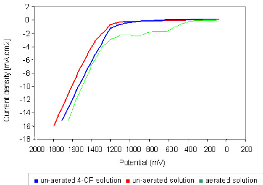
Figure 2. Voltammetry profiles for copper RDE ( 0.2 \text{ cm}^2 ) obtained at 1000 rpm using in 100 \text{ mmol}\cdot\text{L}^{-1} sodium-potassium phosphate buffer pH 6.0 at 25^\circ\text{C} with a 150 \text{ mV}\cdot\text{s}^{-1} scan rate.
